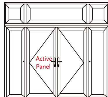
LXFD-OXXOTL Double Opening With Sidelites Fixed Swing Door, w/ Picture at Top.
