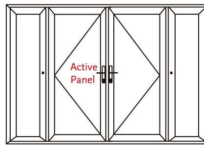
LXFD-OXXOL Double Opening French Door With Sidelites fixed.
